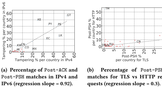
Figure 7: IPv4 vs IPv6 & TLS vs HTTP Tampering.
