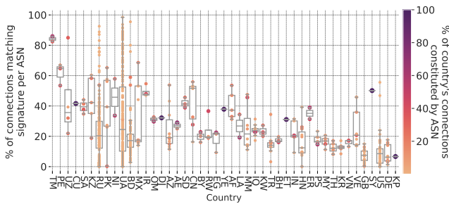
Figure 5: Percentage of connections that match any signature in each large AS (originating the top 80% of connections in a country) in select countries : Each dot represents an ASN and the color reflects percentage of country’s traffic originating from that ASN. Entries on the x -axis mirror Figure 4.
