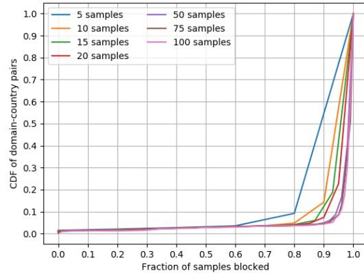
Figure 1: Consistency for various sample rates. This CDF shows the consistency of geoblocking for different sample rates for domain-country pairs we expect to see a geoblock page. (see Section 4.2). A sample size of 20, which we use to confirm geoblocking, yielded only 3.9% of domain-country pairs with less than an 80% geoblocking rate.
